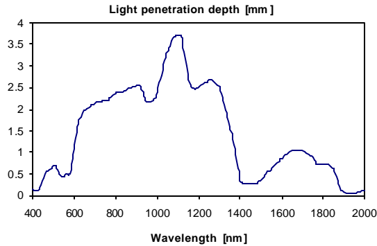
Figure 1. Skin penetration depth of light
