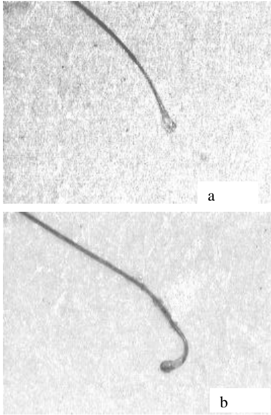
Figure 5 Treated hair a) optical pulse at 20\text{J}/\text{cm}^2 with no additional RF energy. b) optical pulse at 20\text{J}/\text{cm}^2 and RF energy of 20\text{J}/\text{cm}^3 .
